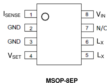
MSOP-8EP
