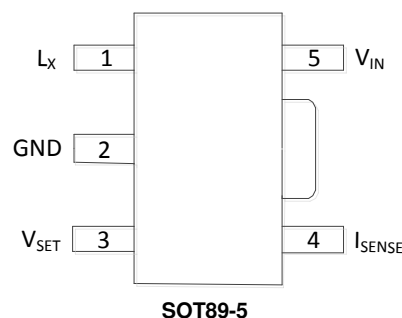
SOT89-5
