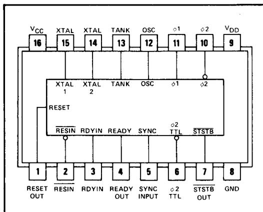
J OR N PACKAGE (TOP VIEW)
