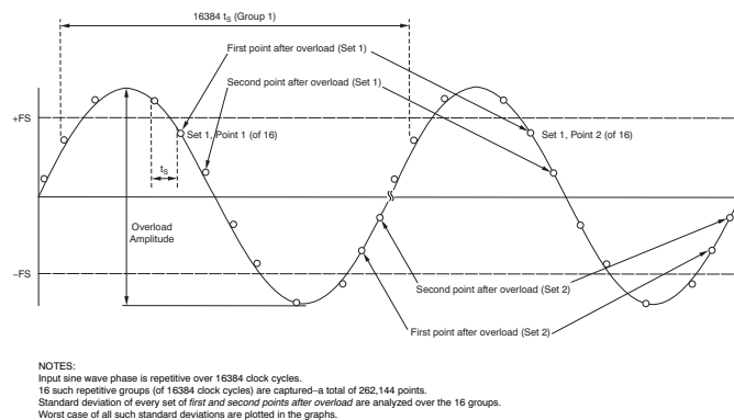
Figure 33. Overload Recovery
