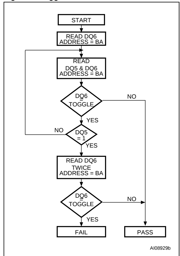
Figure 8. Toggle Flowchart
