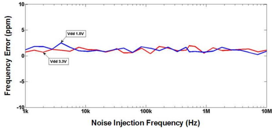
Power Supply Noise Rejection ( \pm 150 mV Noise)
