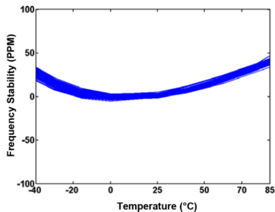
Frequency Stability Over Temperature
