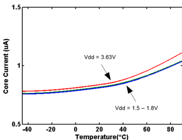
Core Current Over Temperature
