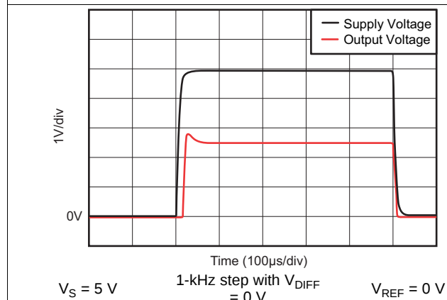
图 21. Start-Up Response
