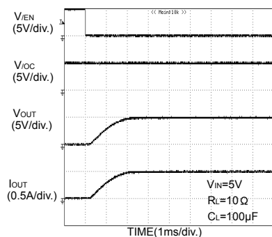
Fig.26 Output rise characteristic (BD2041AFJ)
