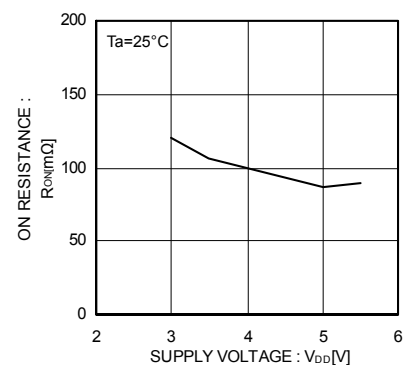
Fig.44 ON resistance
