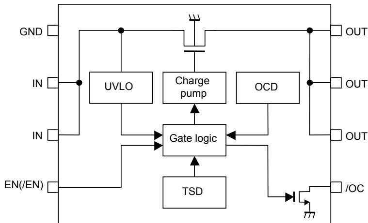
Fig.70 Block diagram
