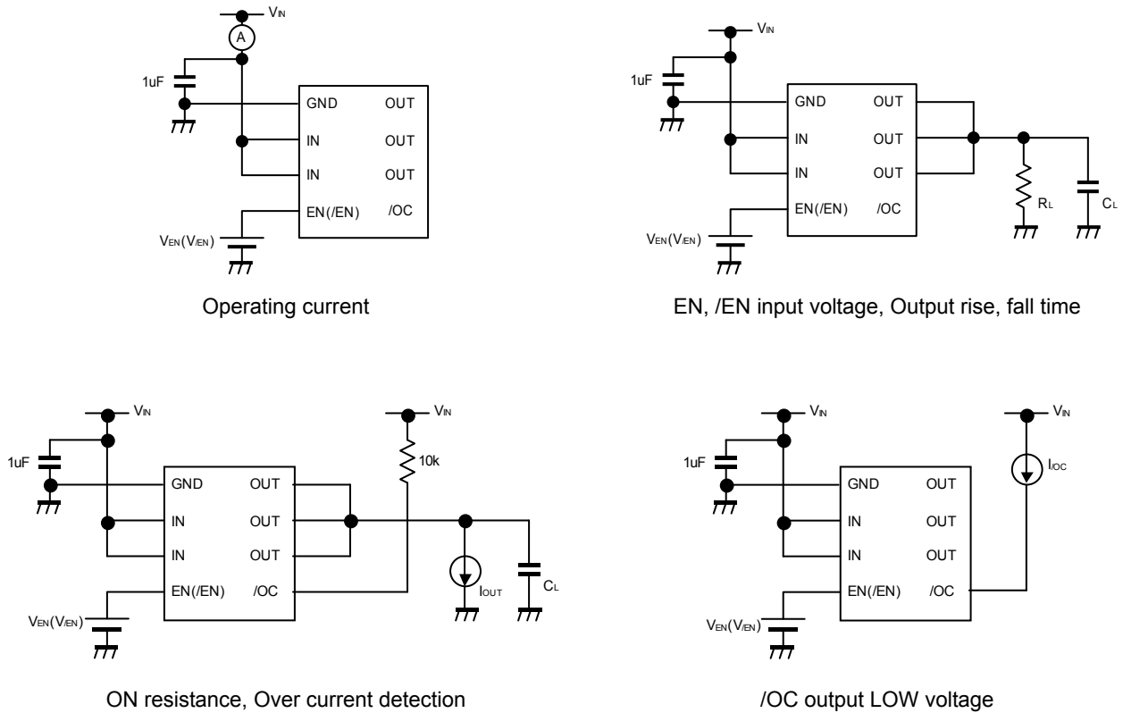
Fig.1 Measurement circuit
