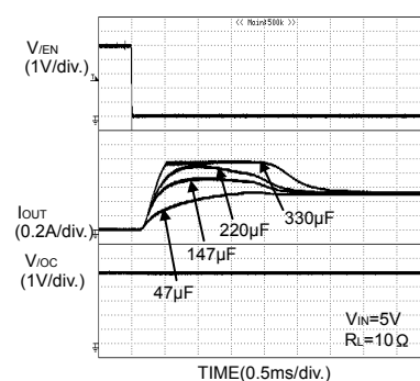
Fig.28 Inrush current (BD2041AFJ)
