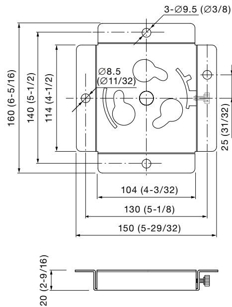
Attachment plate
