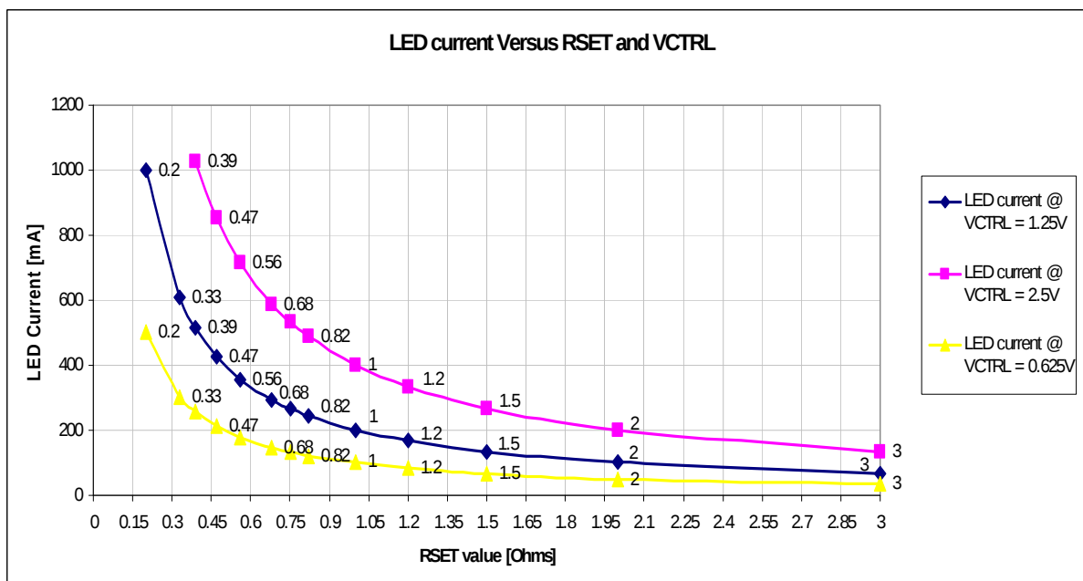
Figure 3: LED Current setting Vs R SET and V CTRL
