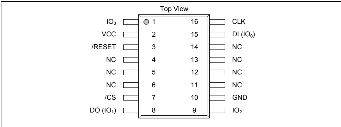
Figure 1c. 16-pin SOIC 300-mil Pin Assignments, 16-pin SOIC 300-mil (Package Code SF)
