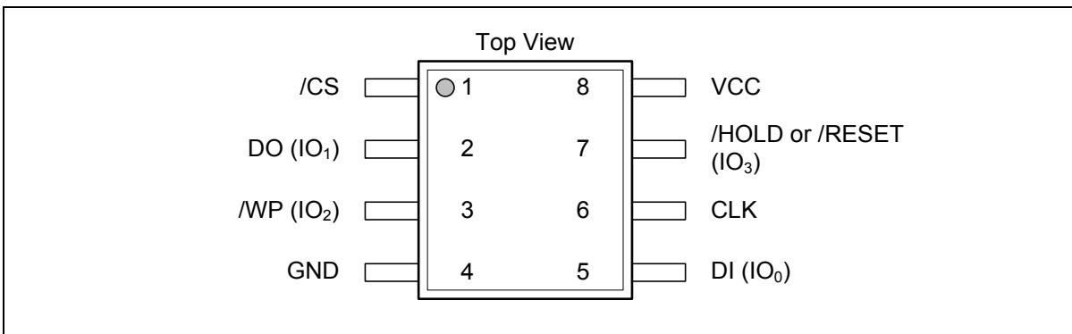
Figure 1a. HM25Q64A Pin Assignments, 8-pin SOIC 208-mil (Package Code SS)
