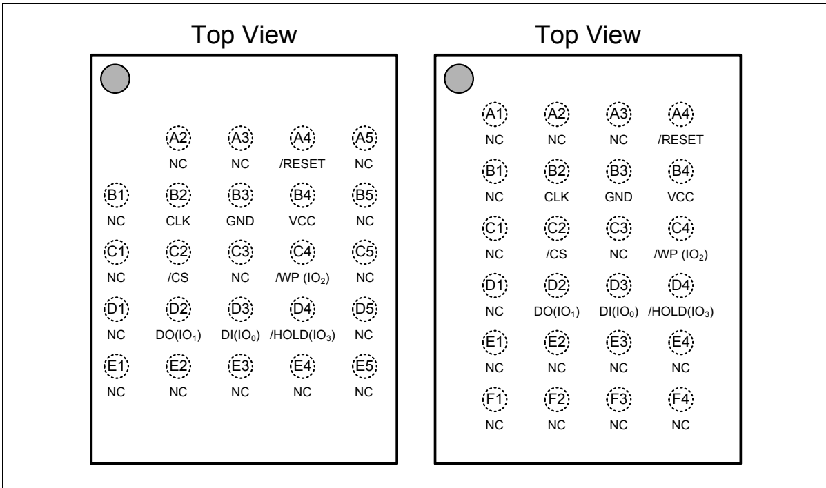
Figure 1d. HM25Q64A Ball Assignments, 24 -ball TFBGA 8x6-mm (Package Code TB/TC)
