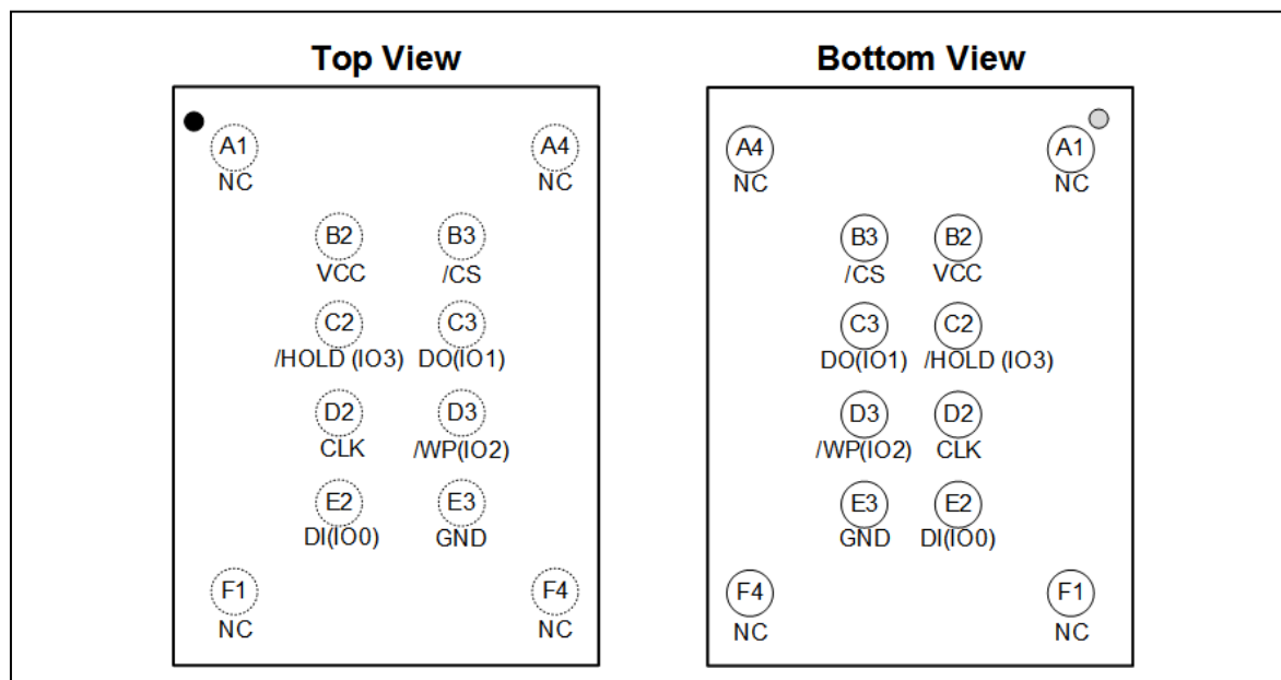
Figure 1e. HM25Q64A Ball Assignments, 12-ball WLCSP (Package Code BY)
