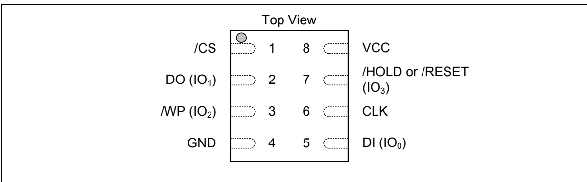
Figure 1b. HM25Q64A Pad Assignments, 8-pad WSON 6x5-mm/8x6 (Package Code ZP, ZE)
