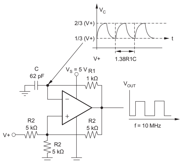
Figure 16. Relaxation Oscillator
