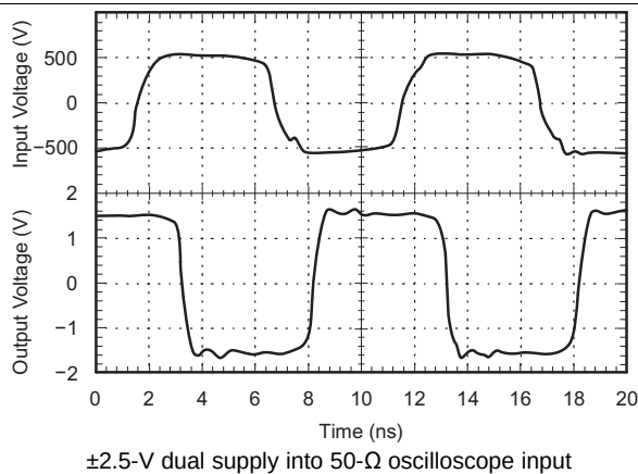
Figure 10. Response to 100 MHz Sine Wave
