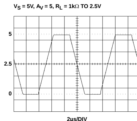
FIGURE 20. OUTPUT SWING
