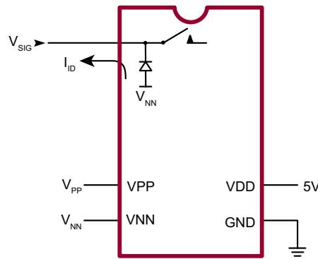
Output Switch Isolation Diode Current
