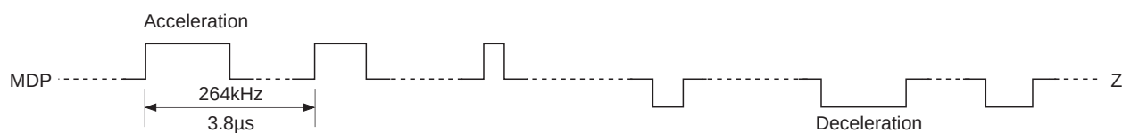
Timing Chart 1-9
