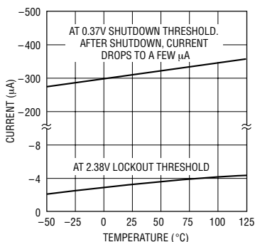
关断引脚偏置电流
