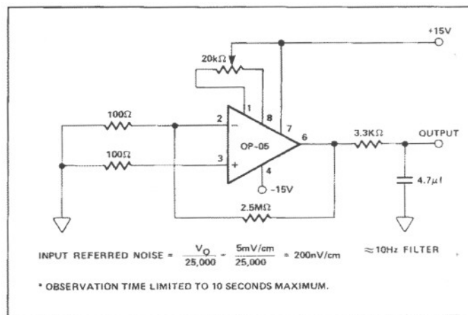
TYPICAL LOW-FREQUENCY NOISE TEST CIRCUIT*
