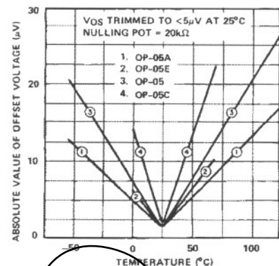
TRIMMED OFFSET VOLTAGE vs TEMPERATURE
