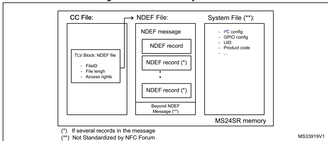
Figure 4. M24SR memory overview
