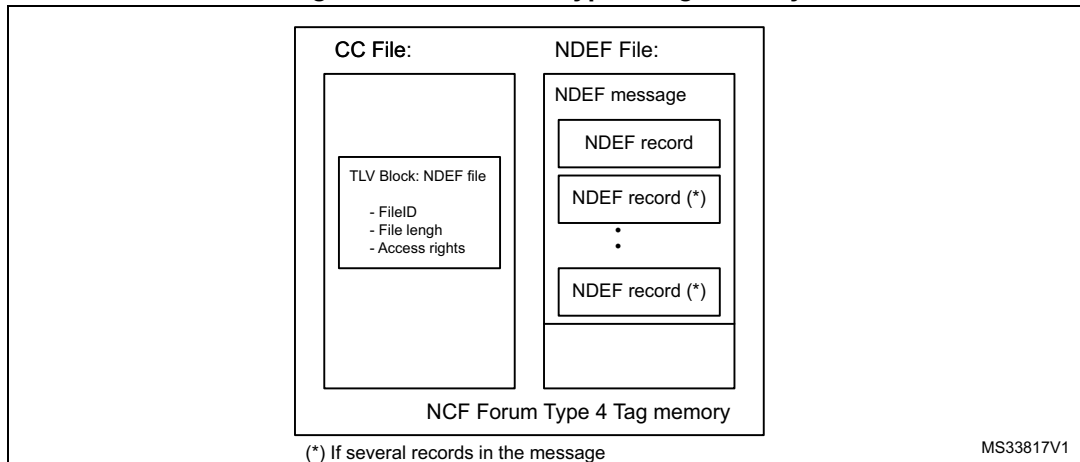
Figure 2. NFC Forum Type 4 Tag memory
