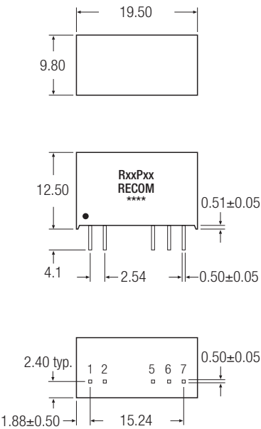
7 Pin SIP Package Style
