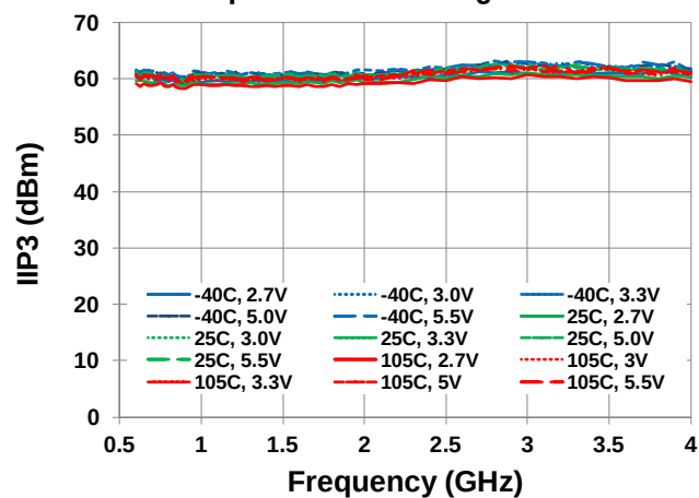
RFX IIP3 vs. Temperature and Voltage
