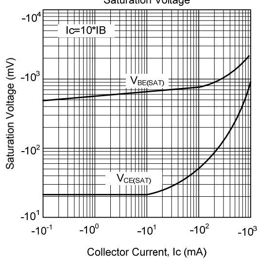
Saturation Voltage
