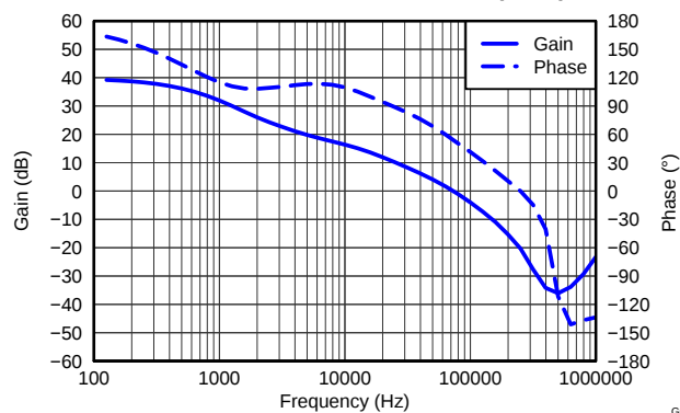
CLOSED LOOP RESPONSE, VIN (3.3 V), 4 A
