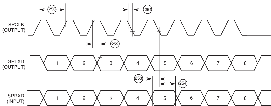
Figure 22. Serial Communication Port Timing Diagram
