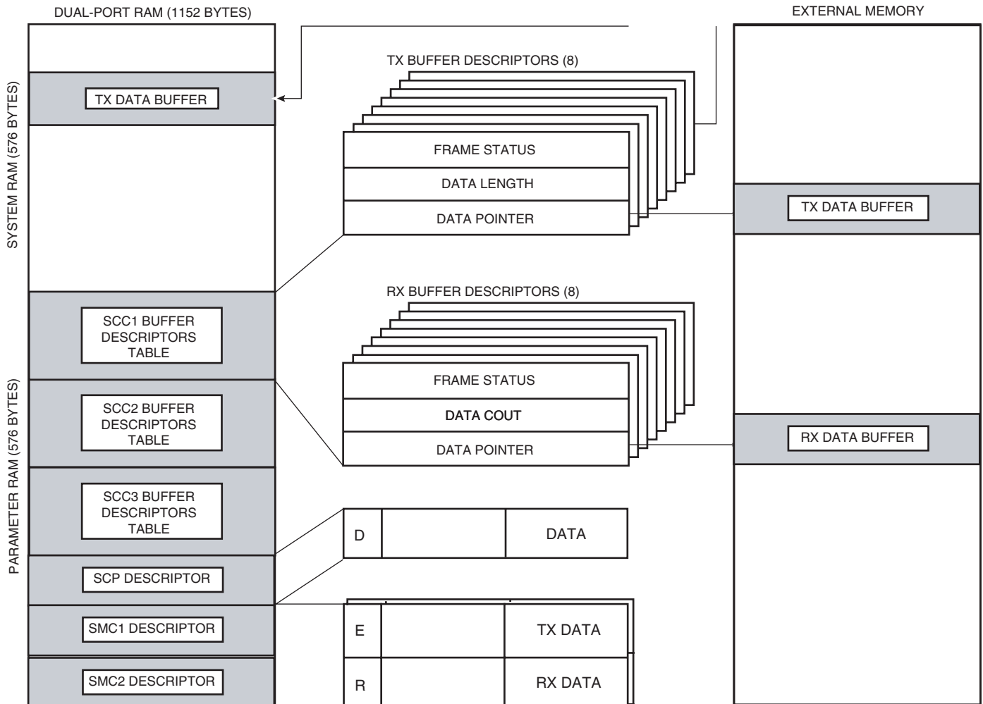
Figure 27. Buffer Memory Structure
