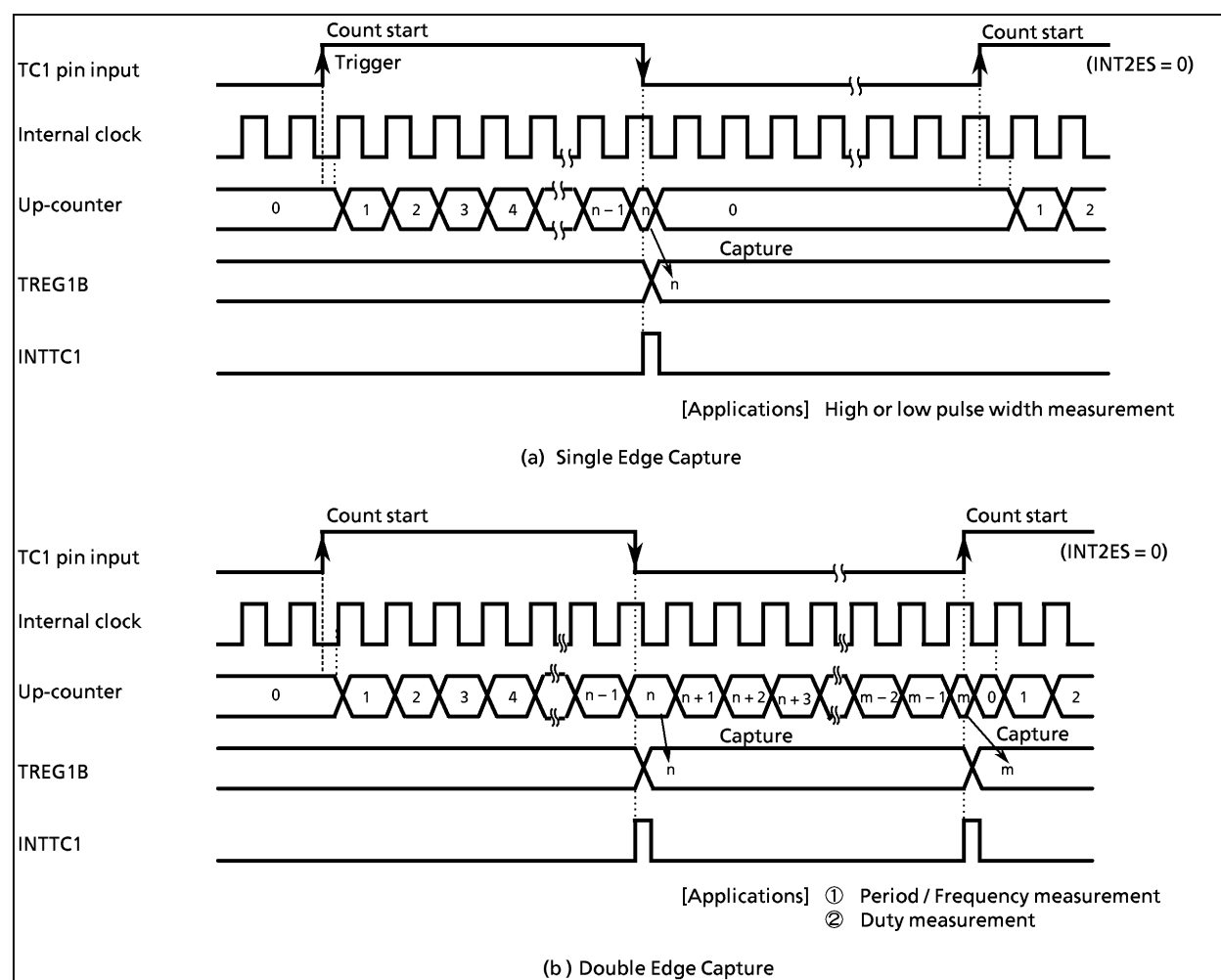
Figure 2-20. Pulse Width Measurement Mode Timing Chart
