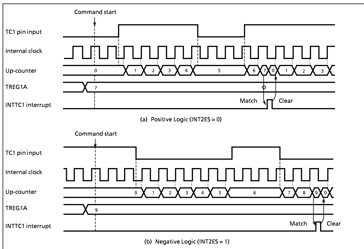
Figure 2-19. Window Mode Timing Chart
