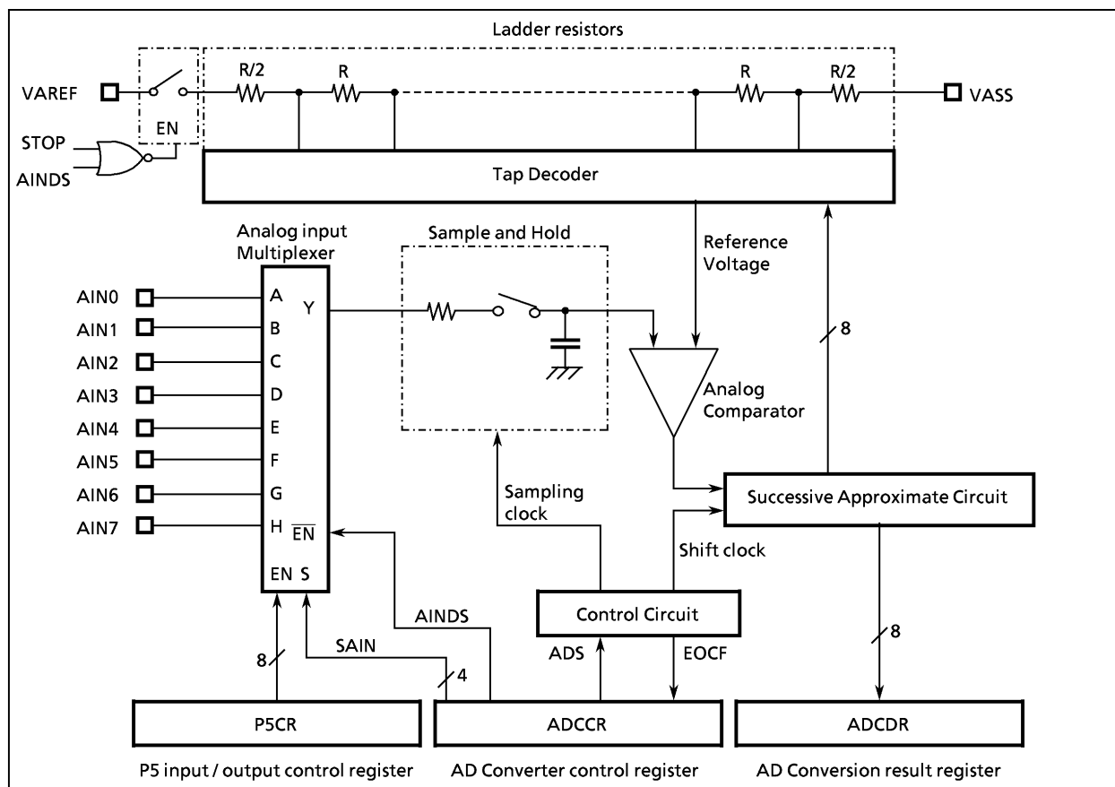
Figure 2-55. AD Converter
