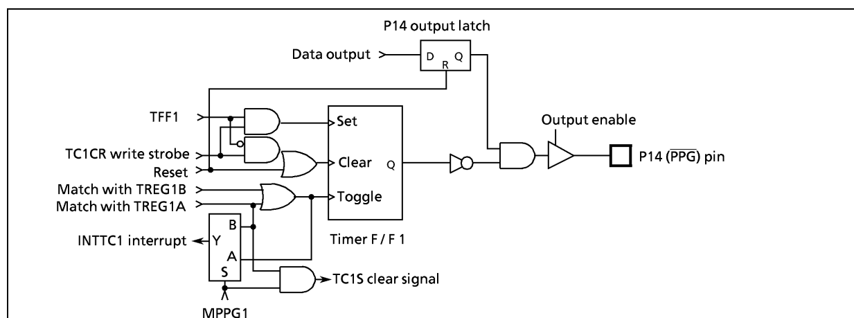
Figure 2-21. \overline{\text{PPG}} Output
