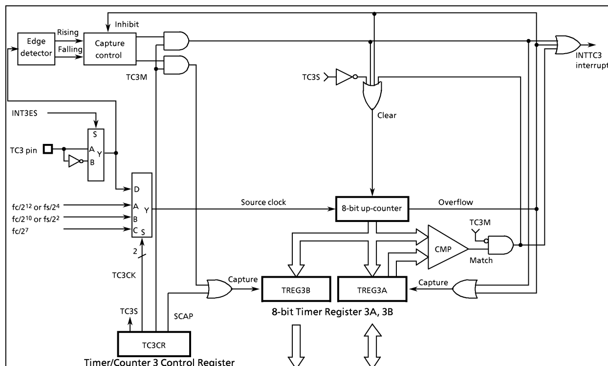
Figure 2-26. Timer/Counter 3
