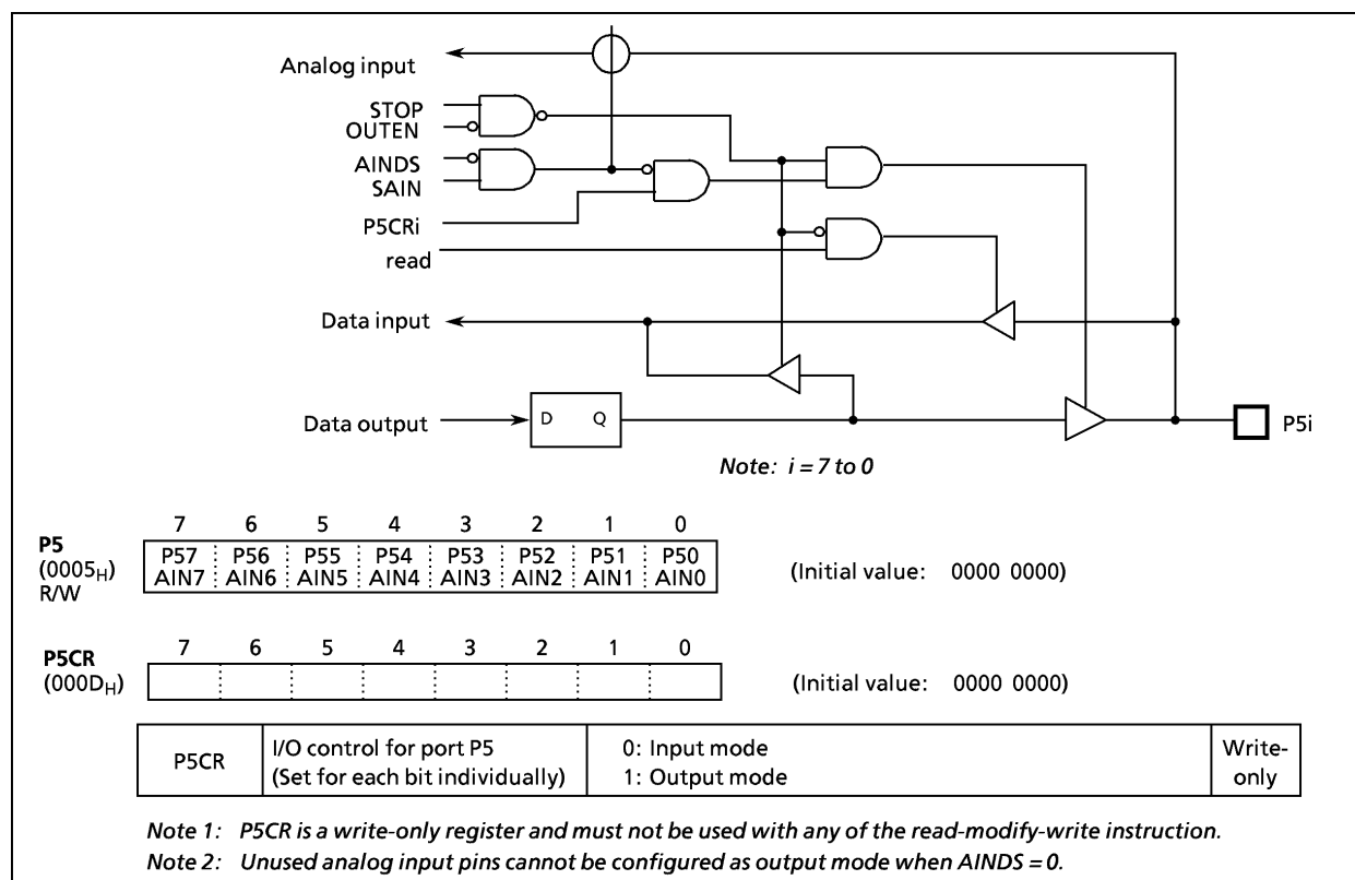
Figure 2-8. Port P5
