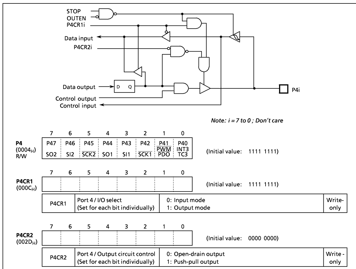
Figure 2-7. Port P4
