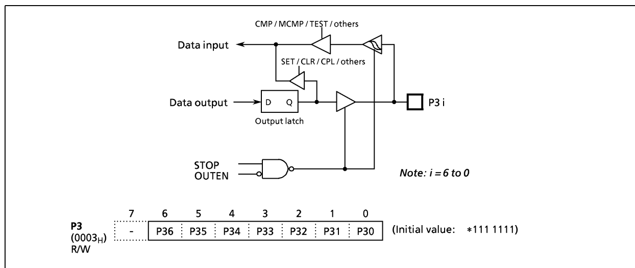
Figure 2-6. Port P3
