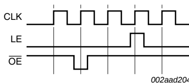
Fig 6. Timing for 'Enter Error Detect Mode' command
