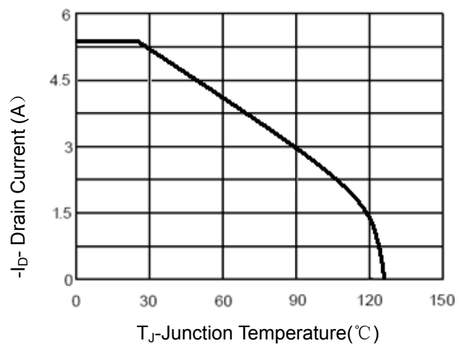
Figure 4 Drain Current
