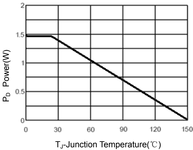
Figure 3 Power Dissipation
