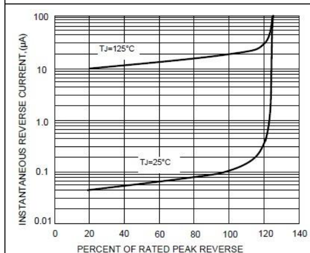
FIG. 5 PERCENT OF RATED PEAK REVERSE
