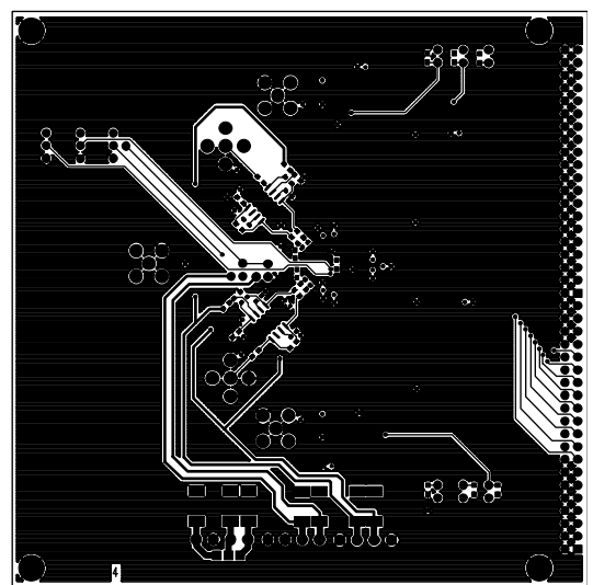
Figure 32. Bottom Routing
