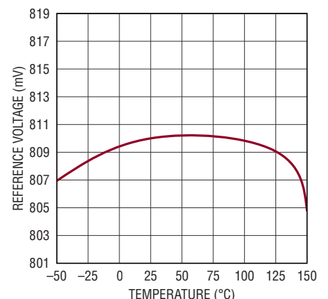
Reference Voltage
