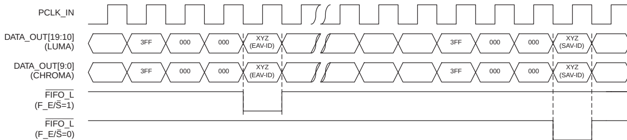
Fig. 4 FIFO_L Timing
