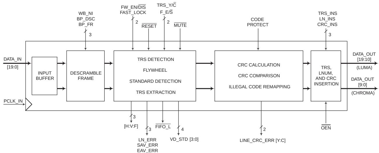
BLOCK DIAGRAM
