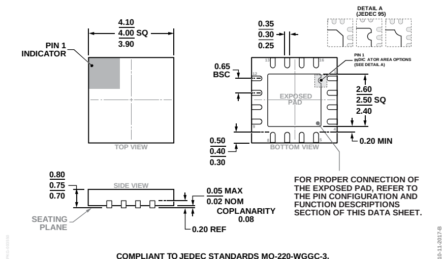
Figure 48. 16-Lead Lead Frame Chip Scale Package [LF CSP] 4 mm x 4 mm Body and 0.75 mm Package Height (CP-16-26) Dimensions shown in millimeters
