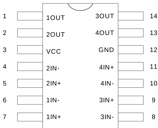
14 Pin PDIP/SOP (Top View)
