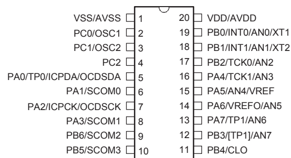
HT66F317/HT66V317 20 SOP-A/SSOP-A
