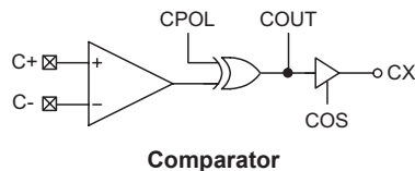
Comparator
