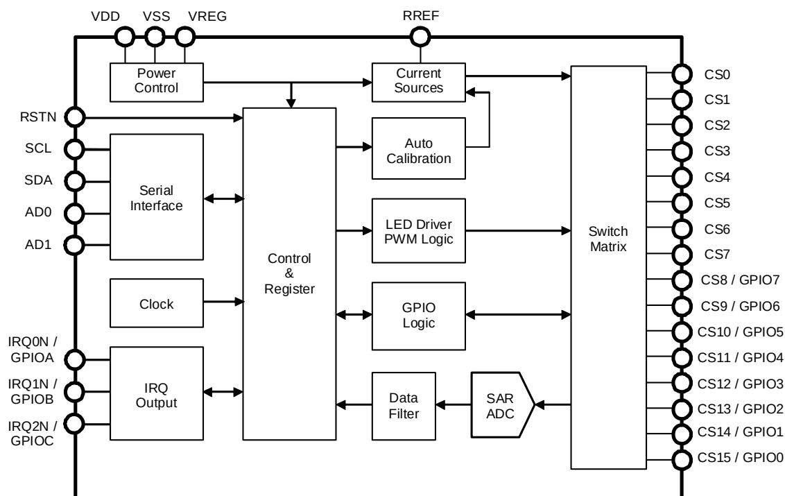
Figure 1. Block Diagram
