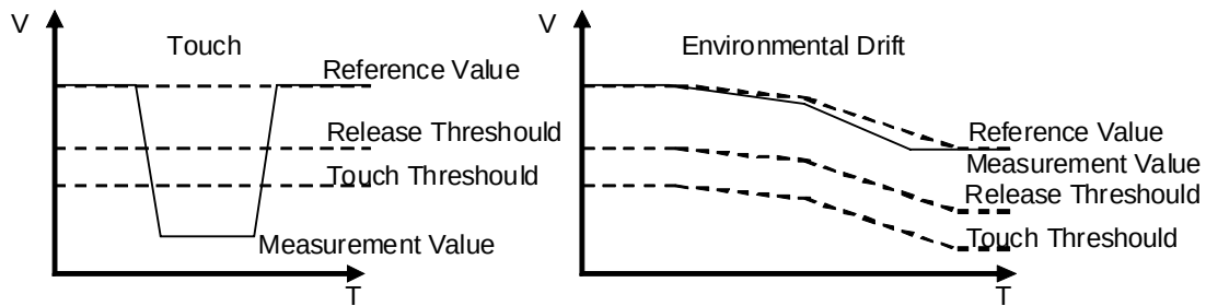
Figure 8. The Voltage of Sense Terminal and Automatic Correction of Environmental Drift
