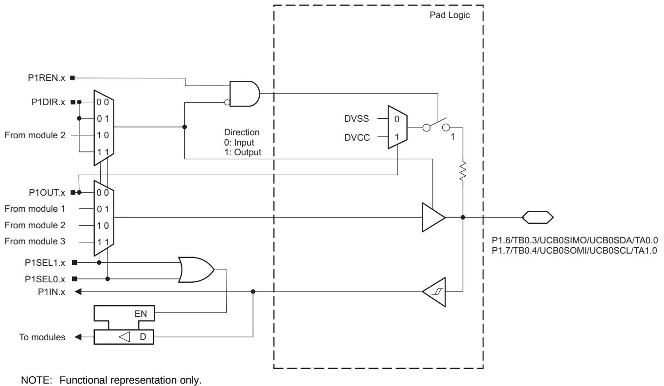
Figure 6-5. Port P1 (P1.6 and P1.7) Schematic
