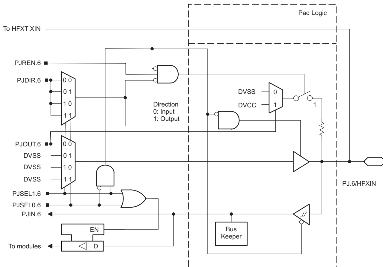
Figure 6-21. Port PJ (PJ.6) Schematic
