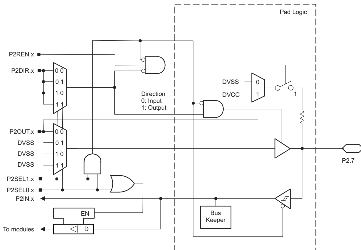
Figure 6-9. Port P2 (P2.7) Schematic
