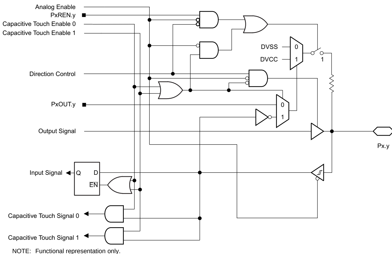
Figure 6-2. Capacitive Touch Functionality on Ports
