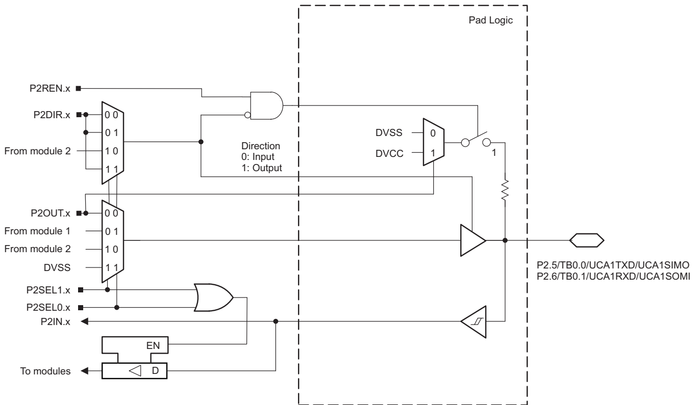
Figure 6-8. Port P2 (P2.5 and P2.6) Schematic
