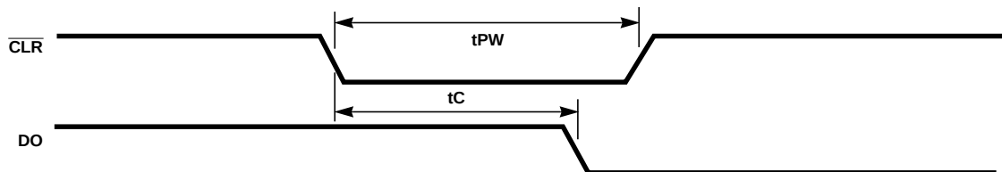
FIGURE 5. CLEAR TIMING
