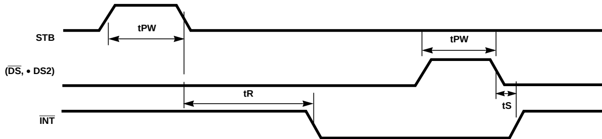
FIGURE 4. INTERRUPT TIMING
