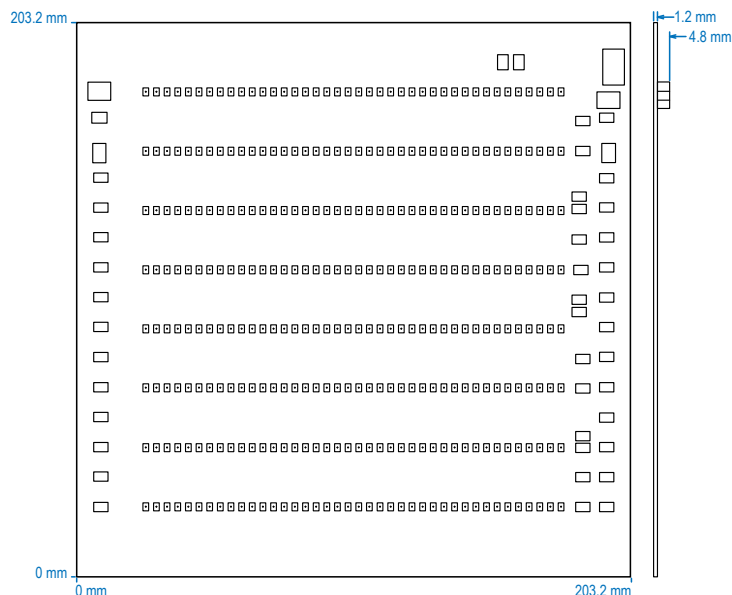
"Warm Dimming" 204mm 120V AC Square LED Module 114W
