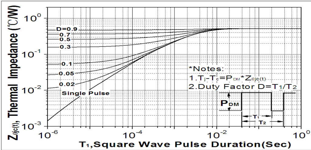
Fig. 12. Transient thermal response curve (TO-251N)
