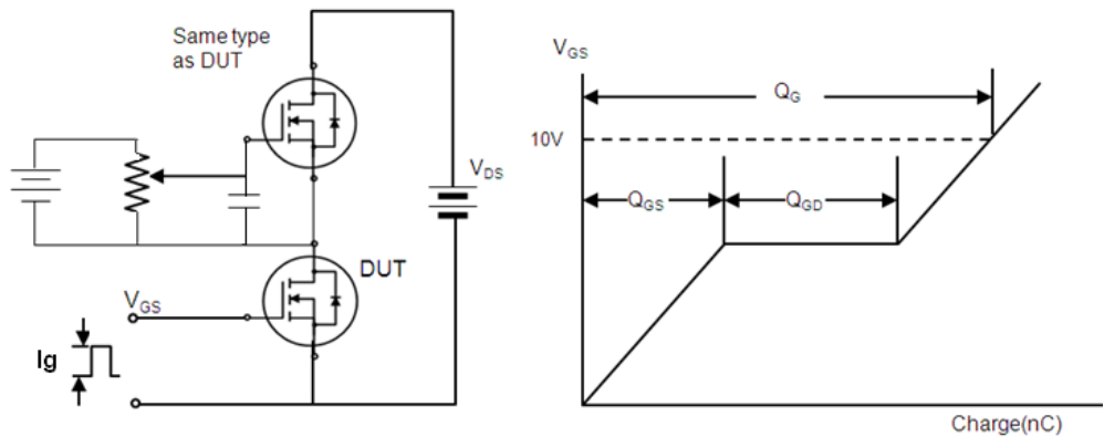
Fig. 13. Gate charge test circuit & waveform
