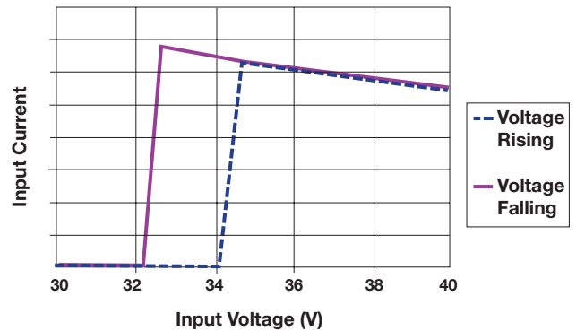
Undervoltage Lockout
