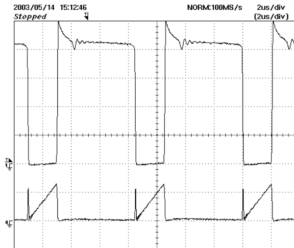
Figure 13 – 230 VAC, Full Load Upper: V_{DRAIN} , 100 V, 2 \mu s / div. Lower: I_{DRAIN} , 0.5 A / div.
