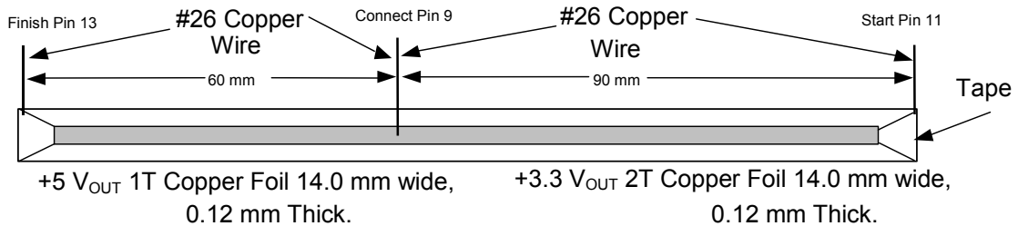
Figure 6 - Copper Foil Winding Information.
