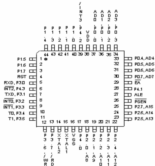
44-Pin QFP
