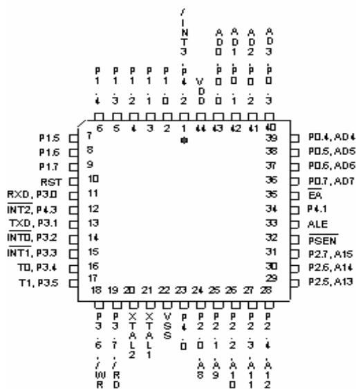
44-Pin PLCC
