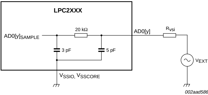
Fig 12. Suggested ADC interface - LPC2470 AD0[y] pin
