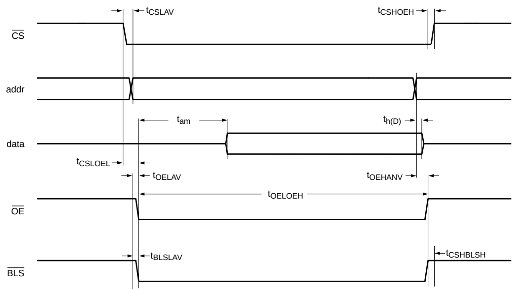
Fig 16. External memory read access
