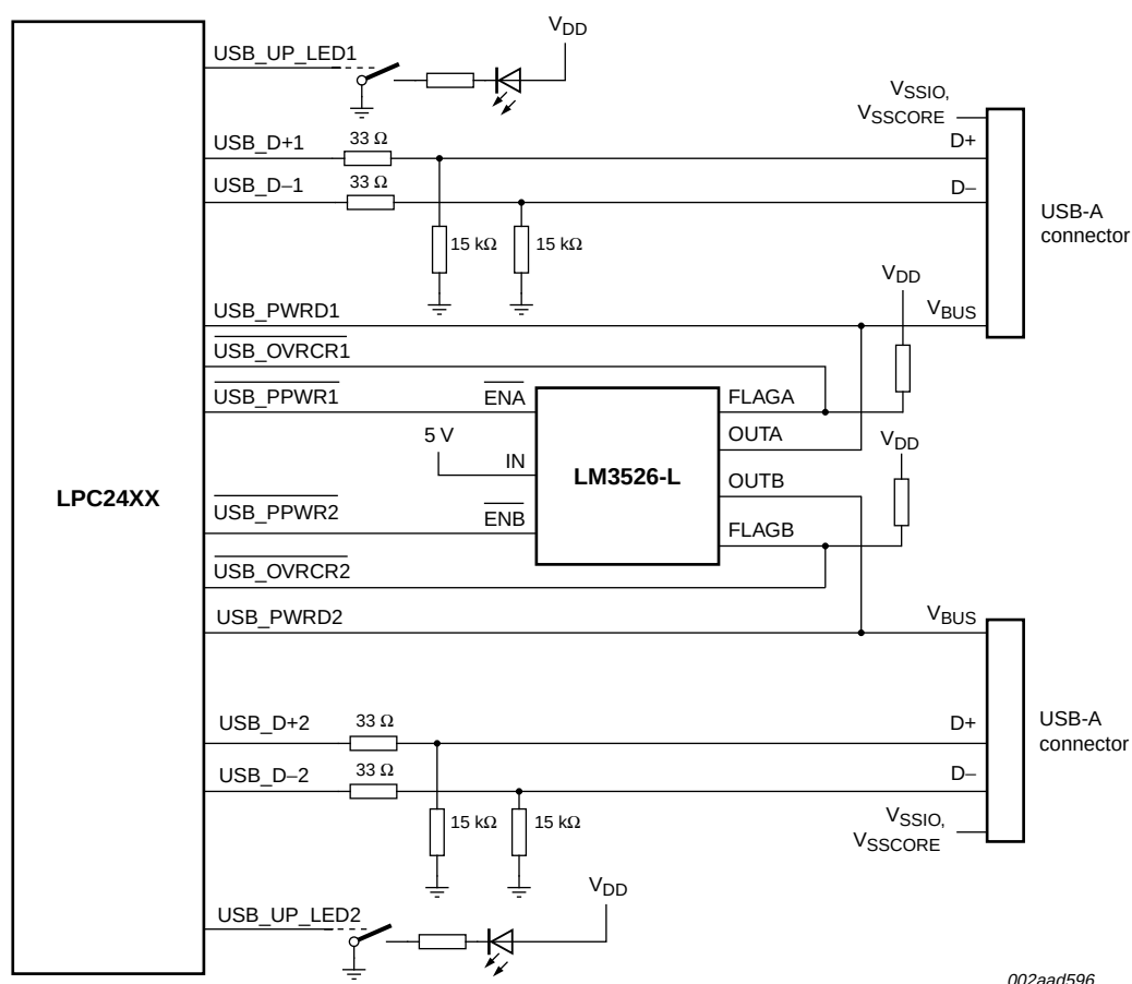
Fig 24. LPC2470 USB OTG port configuration: USB port 1 host, USB port 2 host
