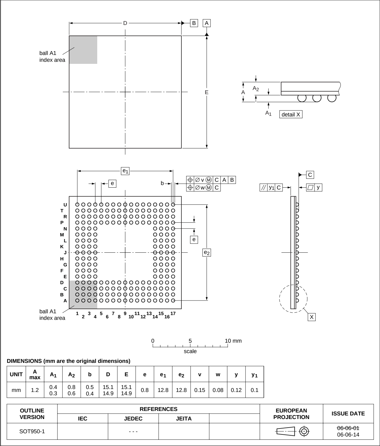
Fig 29. Package outline SOT950-1 (TFBGA208)
