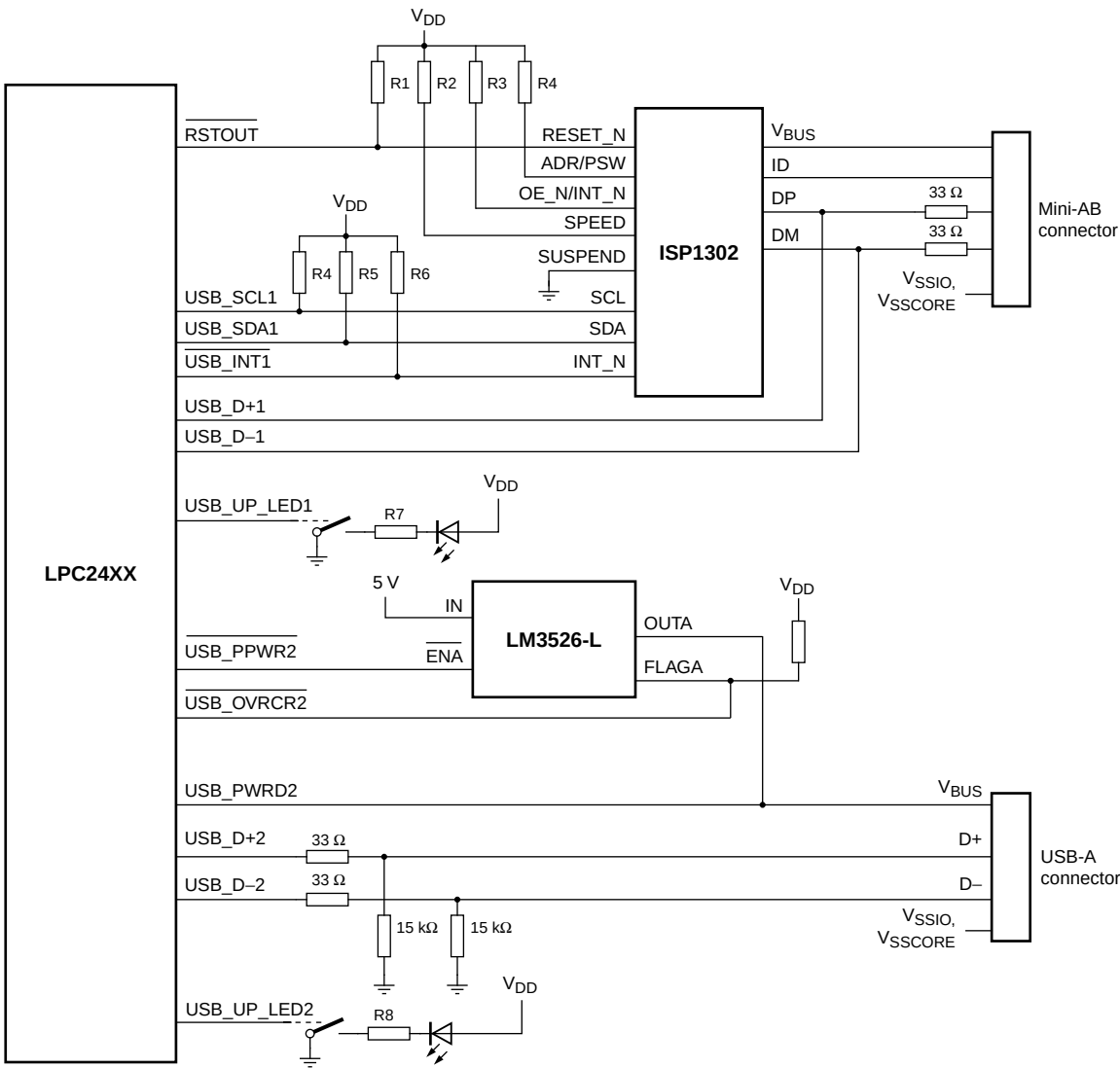
Fig 21. LPC2470 USB OTG port configuration: USB port 1 OTG dual-role device, USB port 2 host
