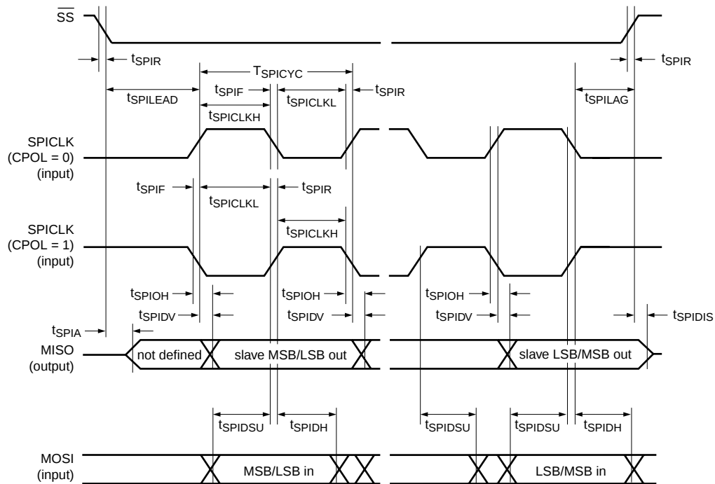
Fig 30. SPI slave timing (CPHA = 1)
