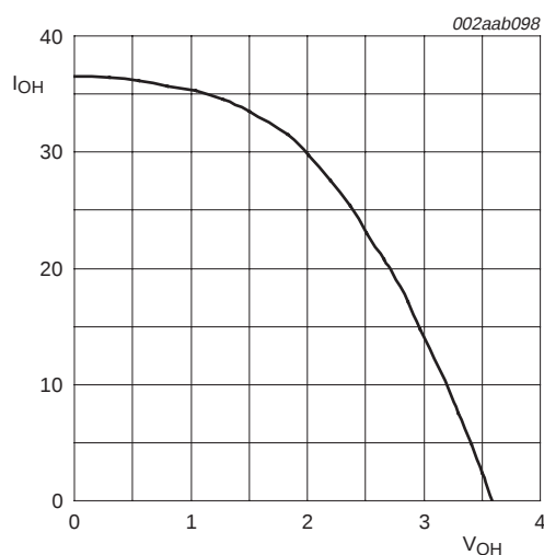
a. T_{amb} = 25^\circ\text{C} ; V_{DD} = 3.6 \text{ V} ; push-pull mode
