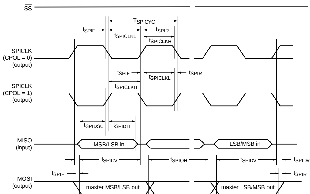
Fig 28. SPI master timing (CPHA = 1)
