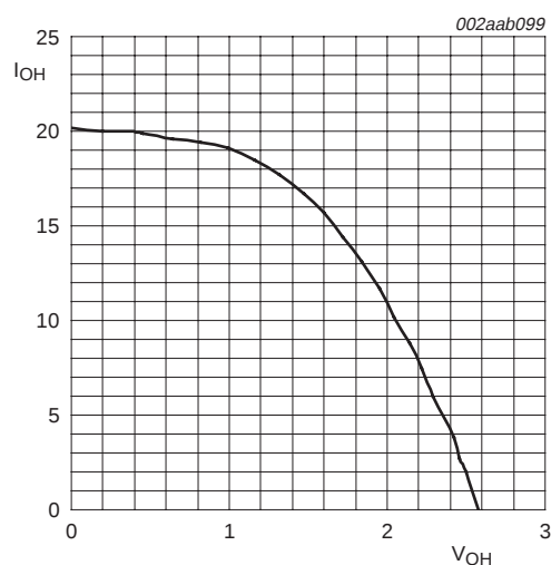
b. T_{amb} = 25^\circ\text{C} ; V_{DD} = 2.6 \text{ V} ; push-pull mode
