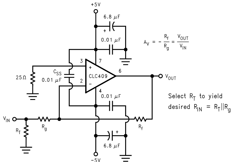
FIGURE 2. Recommended Inverting Gain Circuit
