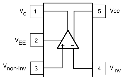
Pinout SOT23-5
