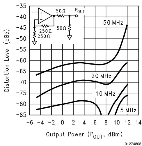
3rd Harmonic Distortion vs. P_{OUT}
