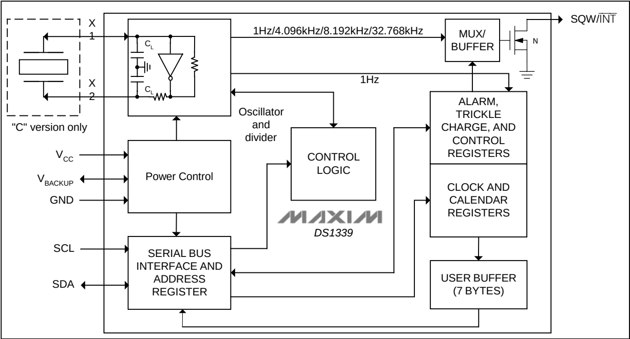
Figure 3. Block Diagram
