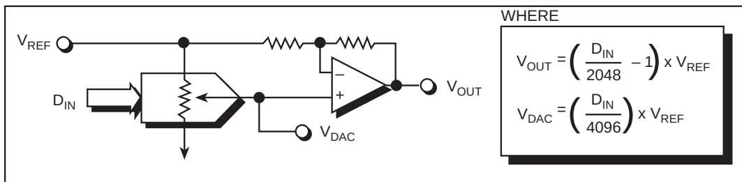
Figure 2. Transfer Function
