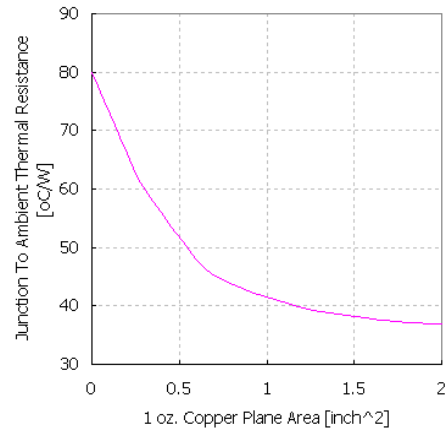
Junction To Ambient Thermal Resistance, \theta_{JA} vs. 1 ounce Copper Area [TO263 Package]
