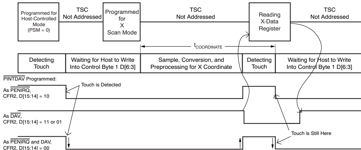
Figure 43. Example of a Single X Coordinate Touch Screen Scan (with Panel Stabilization Time) using TSMODE 3
