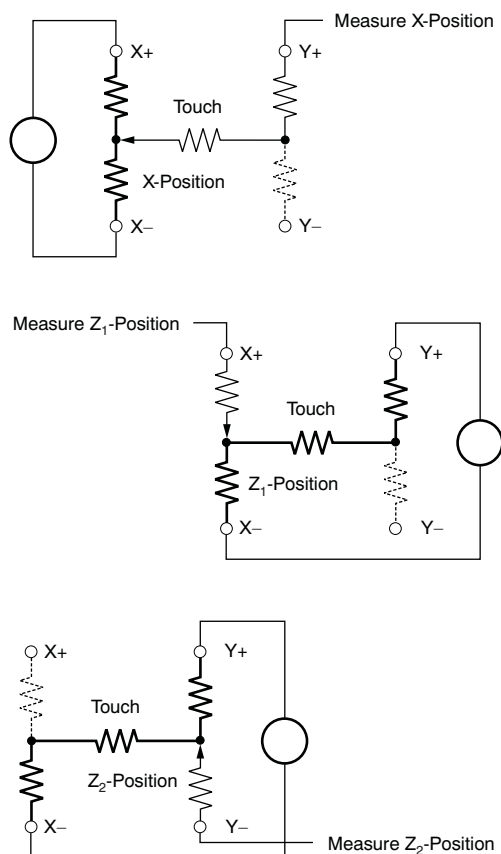
Figure 24. Pressure Measurement
