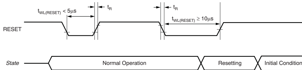
Figure 36. External Reset Timing
