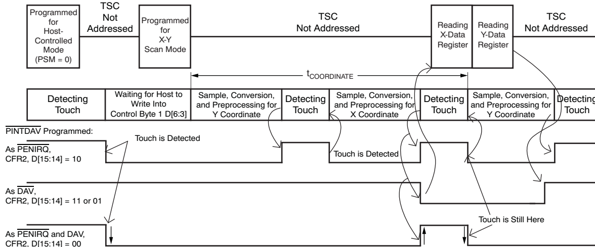
Figure 39. Example of an X and Y Coordinate Touch Screen Scan using TSMODE 2
