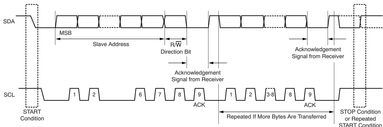
Figure 30. Complete Fast- or Standard-Mode Transfer
