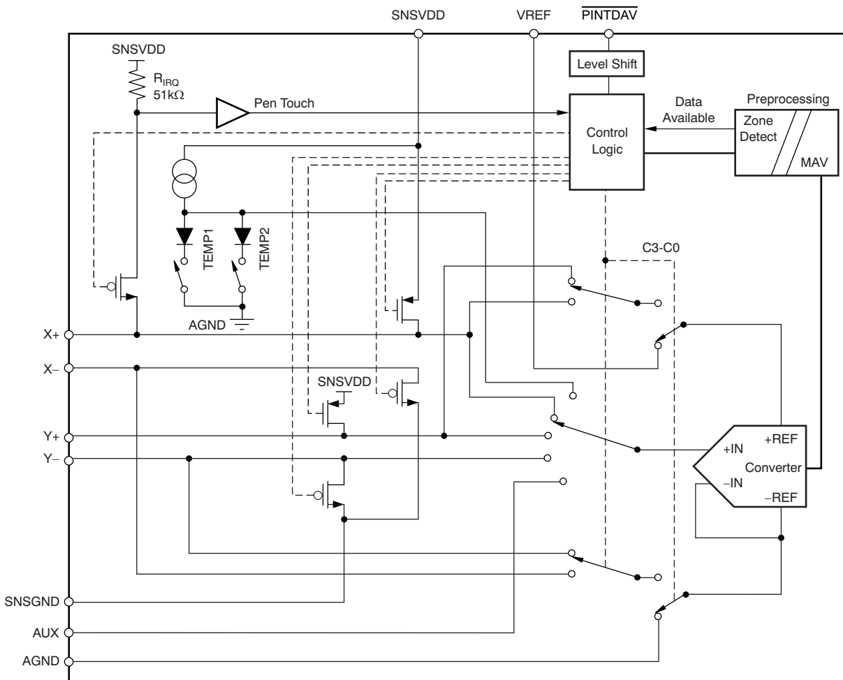
Figure 26. Simplified Diagram of the Analog Input Section
