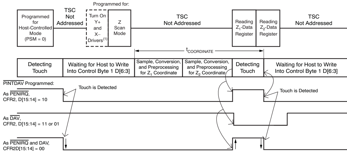
Figure 41. Example of Z_1 and Z_2 Coordinate Touch Screen Scan (without Panel Stabilization Time) using TSMode 3
