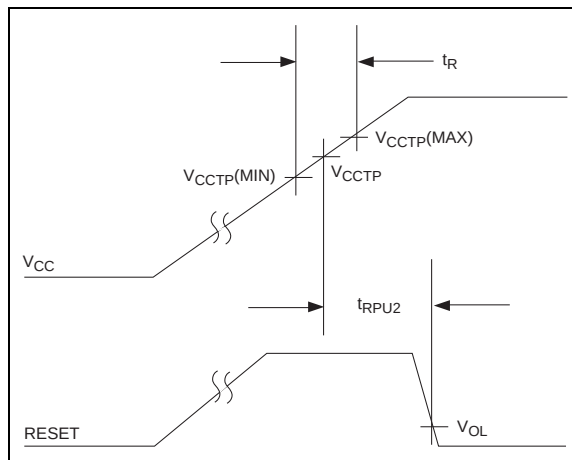
FIGURE 3-3: Timing Diagram – Power Up (TC1277).
