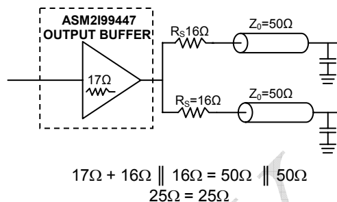
Figure 4. Optimized Dual Line Termination
