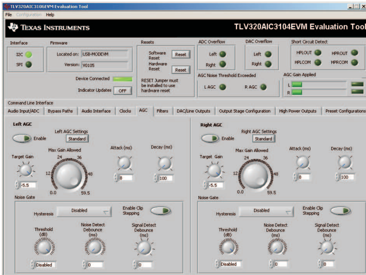
Figure 11. GPIO Tab
